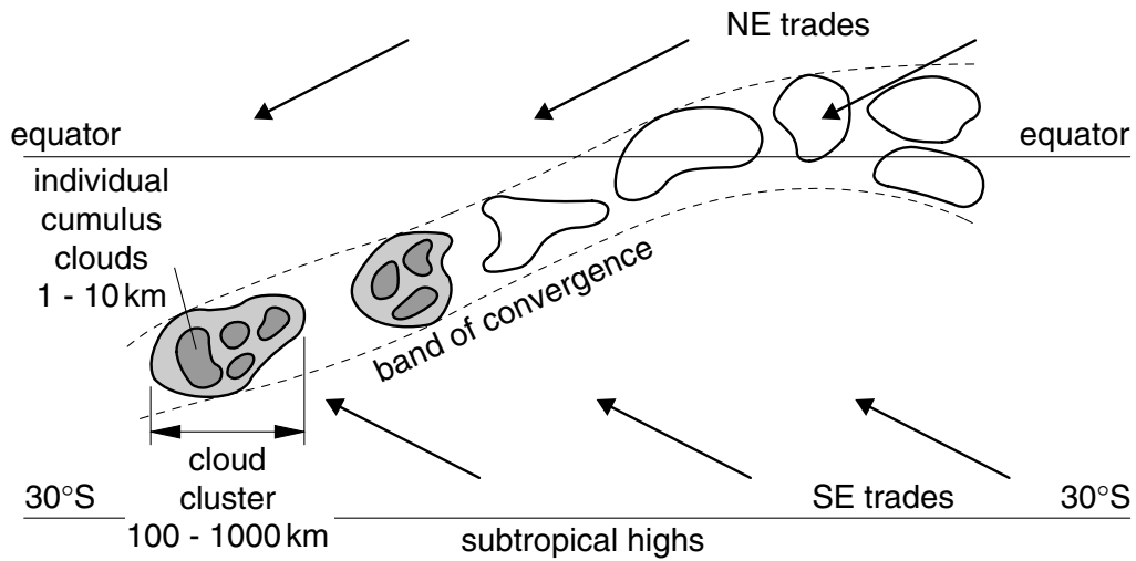
Plan view of the ITCZ
